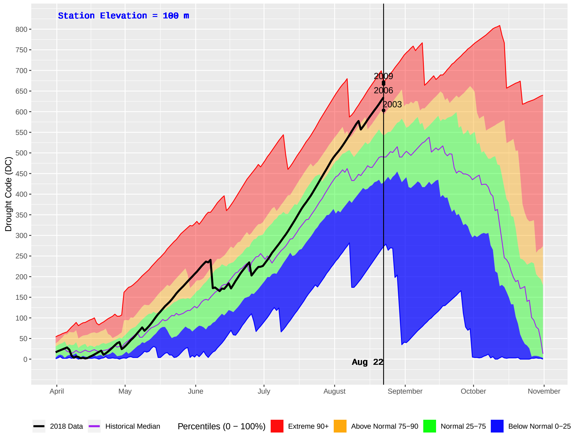
BEAVER CREEK (37) : Historical (1987–2016) and Current (2018) Daily Drought Code (DC)
